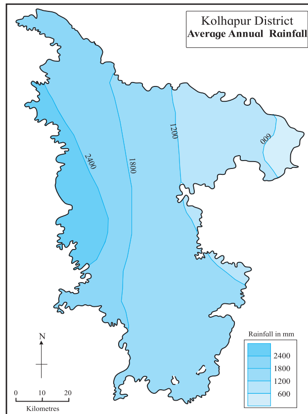
Figure 1.5 : Rainfall
